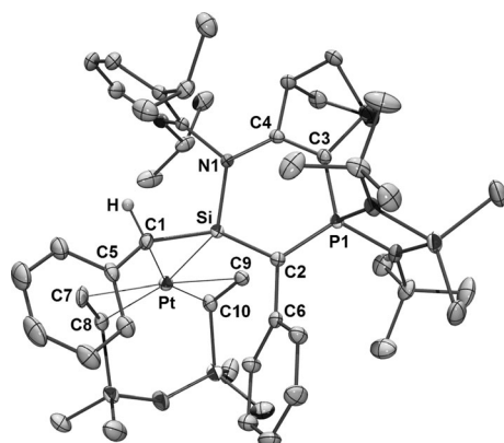
Figure 5. Molecular structure of 11 . Ellipsoids are set at 30% probability; H atoms except for that on C1, disorder and solvent molecule are omitted for clarity. Selected bond lengths [Å] and angles [°]: C1–Si1 1.802(3), Si1–N1 1.772(2), Si1–C2 1.812(3), C1–C5 1.470(4), Si1–Pt 2.440(1), C1–Pt 2.236(3), C2–P1 1.705(3); C1–Si1–Pt 61.47(9), Si1–C1–Pt 73.45(9), C1–Pt–Si1 45.07(7), N1–Si1–C2 110.71(11), C1–Si1–N1 108.92(12), C1–Si1–C2 131.42(13).
